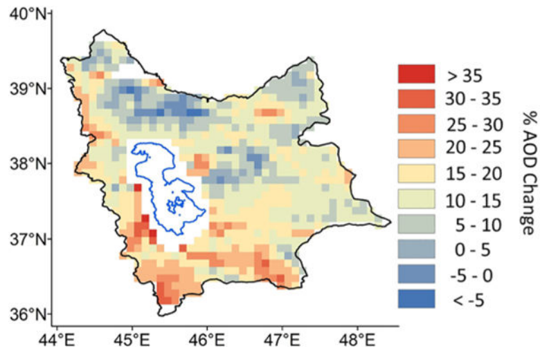
Fig. 6. Spatial distribution of AOD percent change between 2008 and 2015 as compared to 2001–2007. Uncolored pixels represent an insufficient number of data points.
